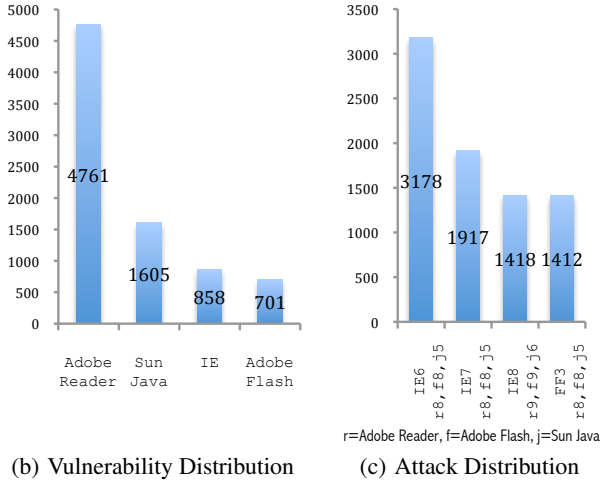
Figure 4: Statistics from daily malicious URL experiment
